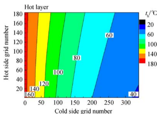
Fig. 9 Temperature distribution of hot layer in wet condition
