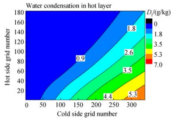
Fig. 12 Condensate distribution
