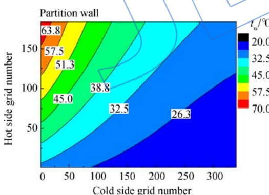
Fig. 8 Temperature distribution of partition wall in dry condition
